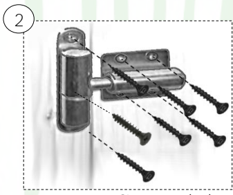
OUTSIDE \text{Ø}3,5 \times 35 (x7)
