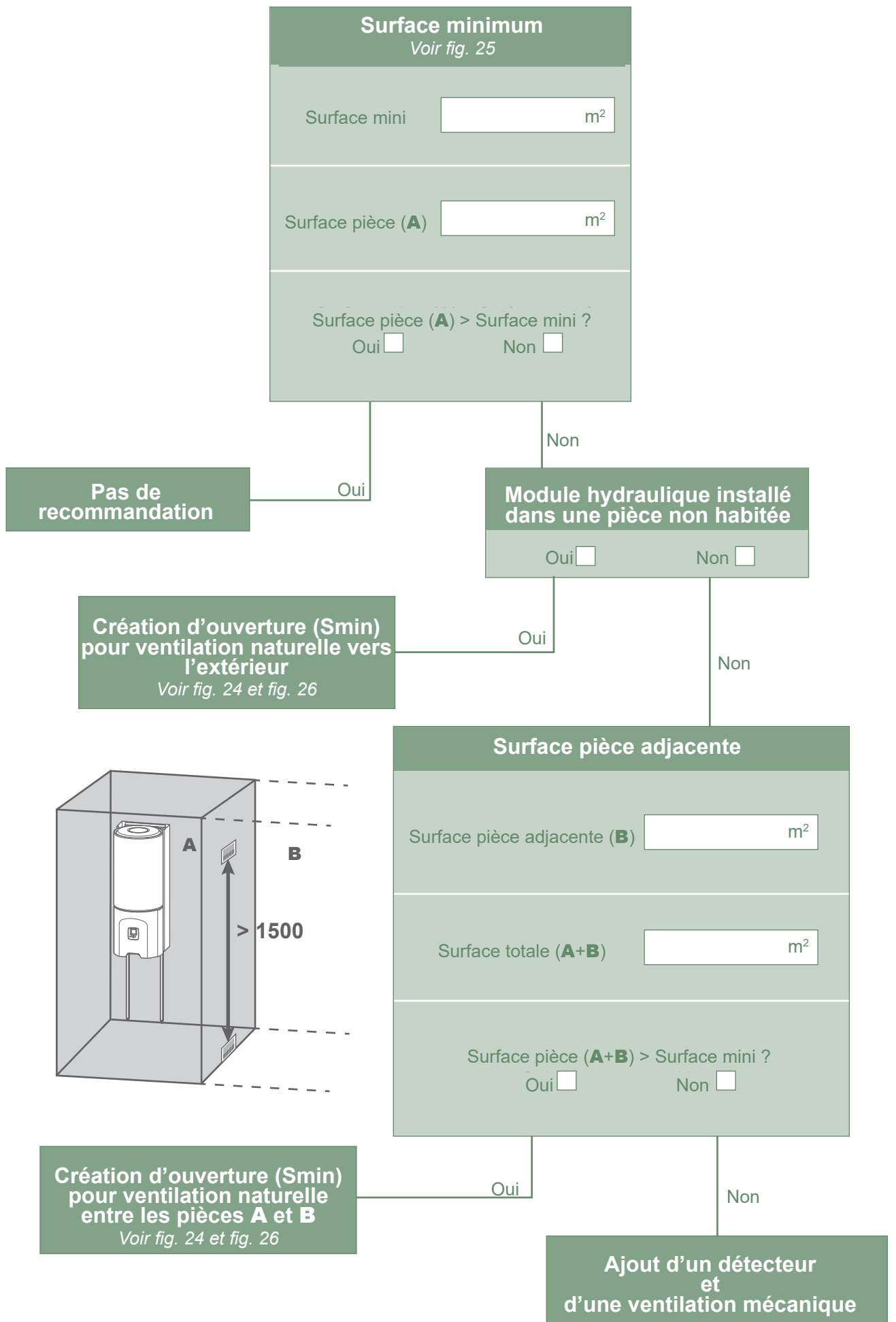
fig. 27 - Surface minimale
