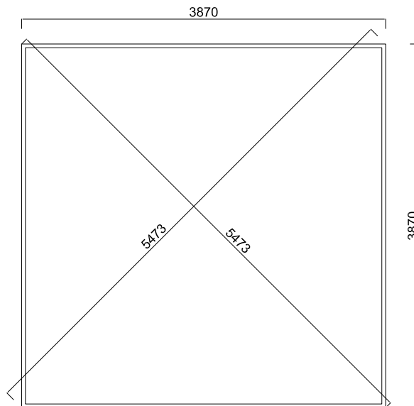
Bottom Beam Dimension Drawing.
