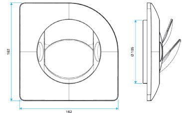
Grille BIO Design carré D 125 mm
