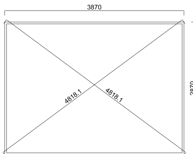
Bottom Beam Dimension Drawing.
