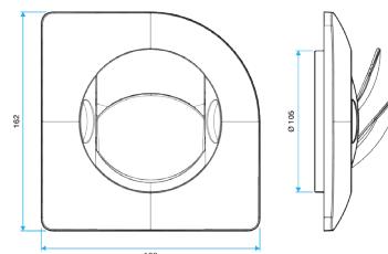
Grille BIO Design carré D 125 mm
